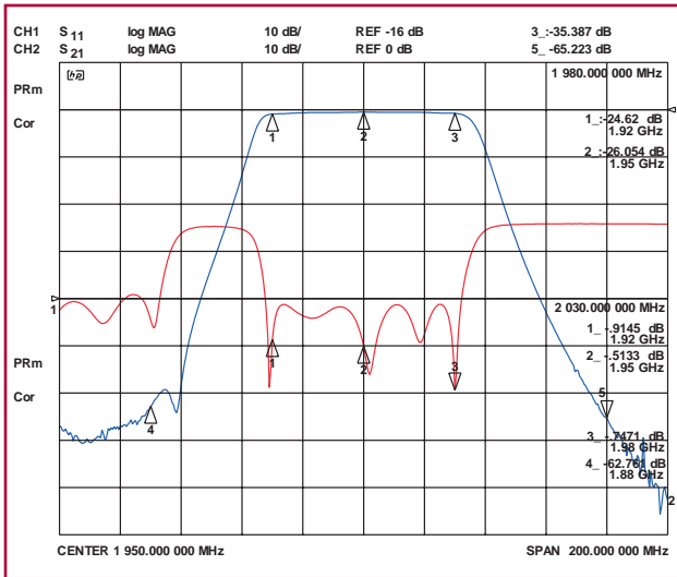
UMTS Receive Response
