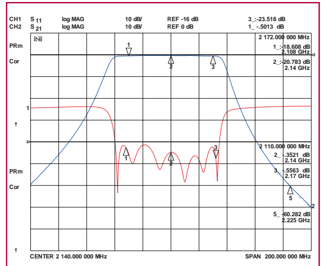
UMTS Transmit Response
