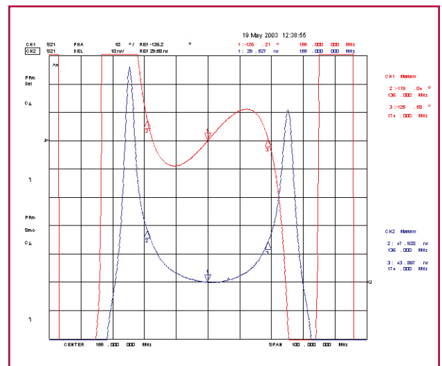
Phase/Group Delay
