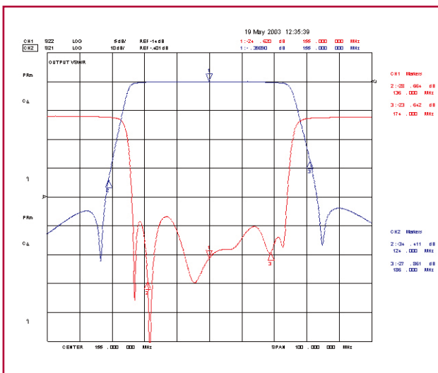
Amplitude/VSWR Response
