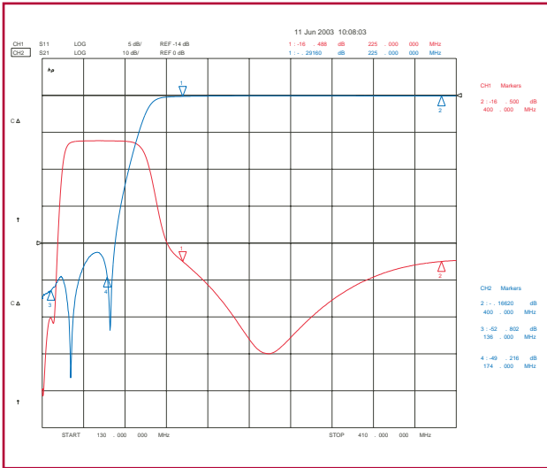
225 to 400 MHz Highpass Filter
