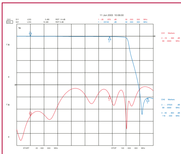
30 to 88 MHz Lowpass Filter
