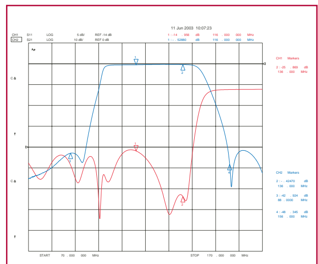
116 to 136 MHz Bandpass Filter
