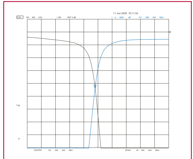
Crossover @ 102 MHz
