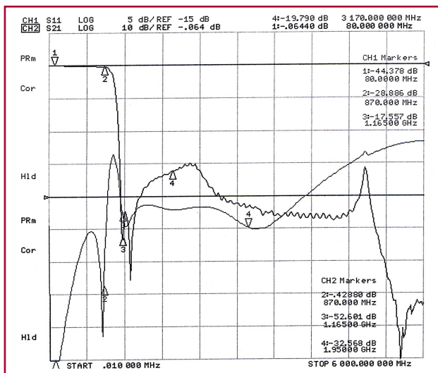
Passband & Return Loss
