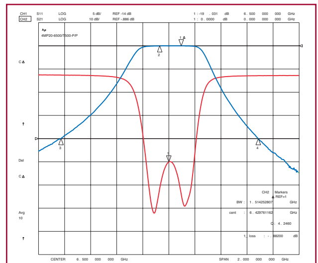
Insertion Return Loss
